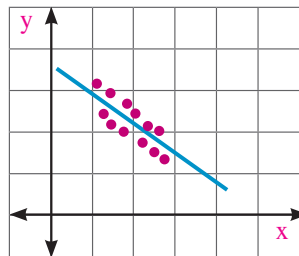
(5) Corrélation indirecte forte
