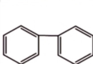
Diphenyl \text{C}_6\text{H}_5\text{-C}_6\text{H}_5
