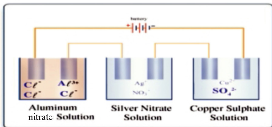
Electrolysis of different electrolytic Solutions (Fig 4-11)
