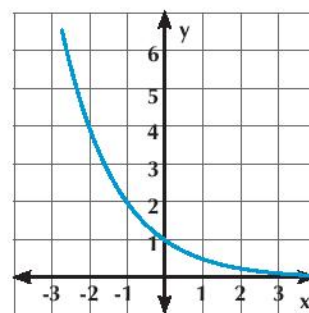
g(x) = \left(\frac{1}{2}\right)^x
