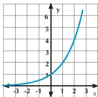
f(x) = 2^x
