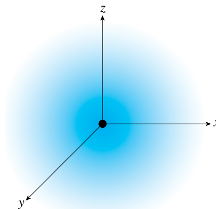
Electron cloud
