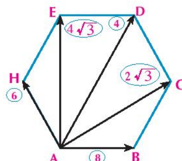
Regular hexagon
