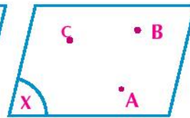
Three distinct and non - collinear points
