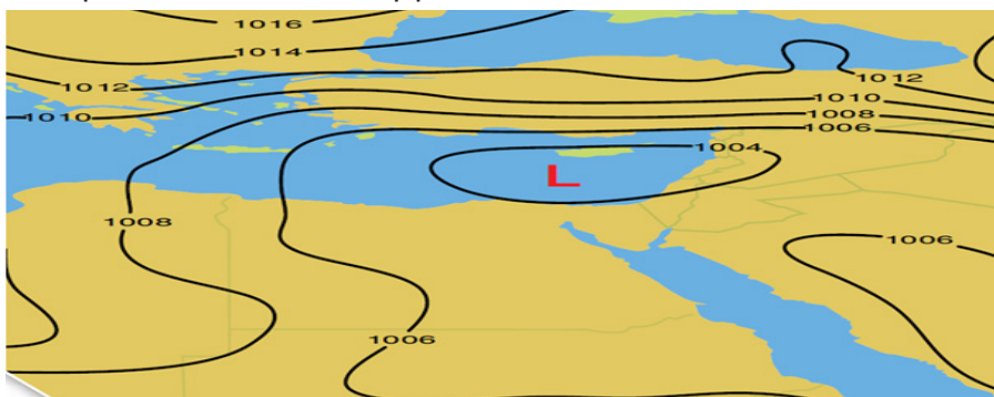
Figure (2-26) lignes isobares
