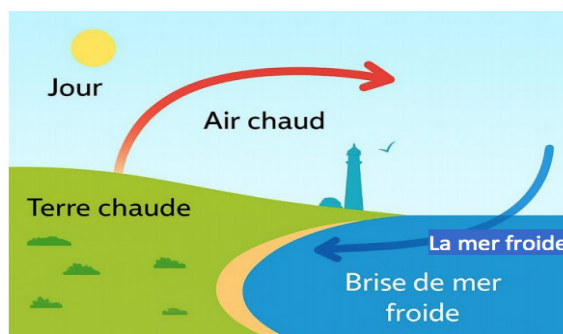
Figure (1-19) la brise de mer
