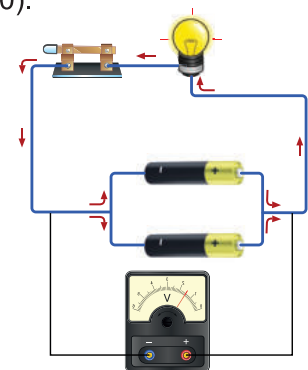
Circuit (3)
