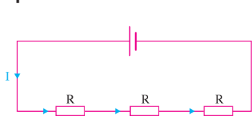
Circuit (1)
