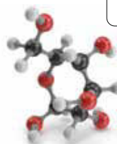
\text{C}_6\text{H}_{12}\text{O}_6
