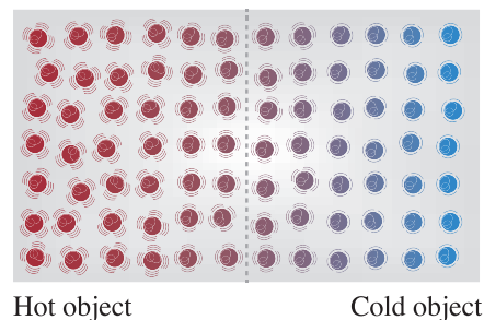
Figure (7) Heat transfer by particle vibration
