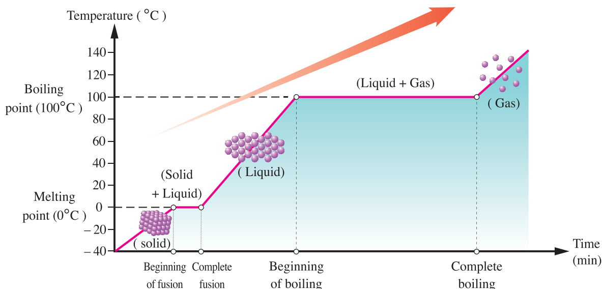
Figure (3) Water heating curve
