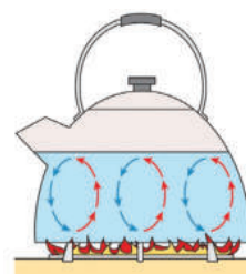
Figure (16) Convection currents
