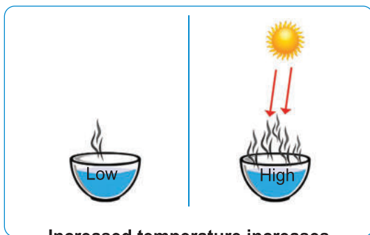
Increased temperature increases the rate of evaporation Figure (14)
