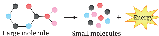
Figure (6) Catabolic process
