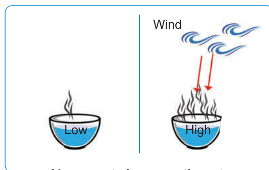
Air currents increase the rate of evaporation Figure (17)
