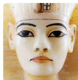
Figure (5) Galena used as eye makeup (kohl) by the ancient Egyptians
