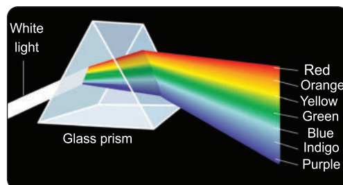
Figure (7) White light is made up of seven colours
