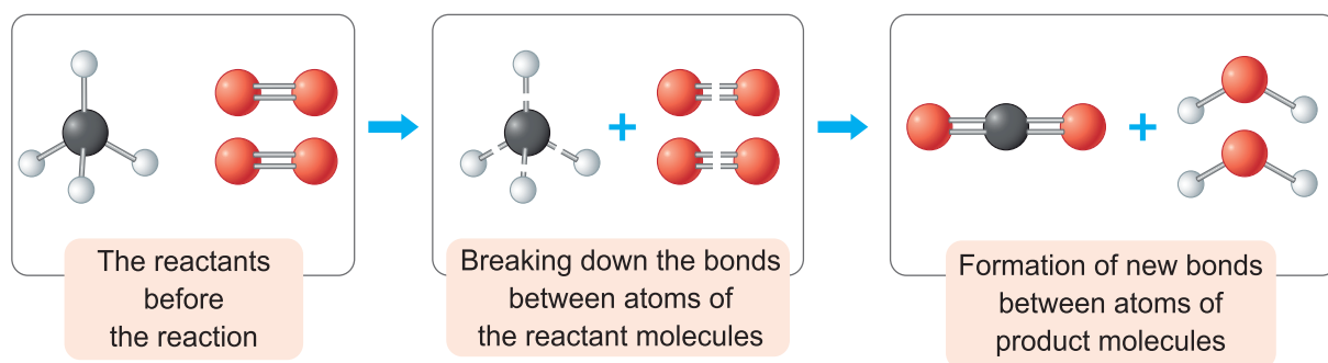
Figure (4) The chemical reaction
