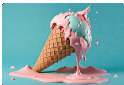
Figure (8) Melting of ice cream by gaining thermal energy
