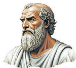
Pythagoras
