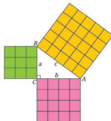
Pythagoras
