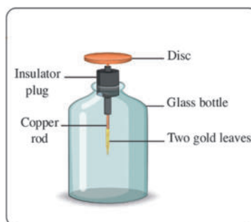
Figure (31) The electroscope
