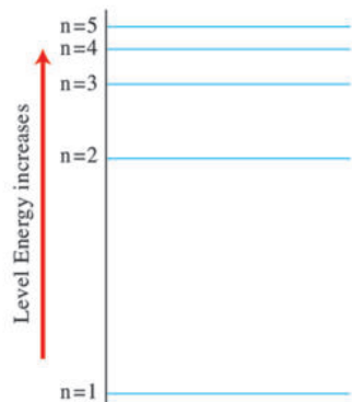
Figure (5) The energy of some levels in which the electrons revolve around the nucleus
