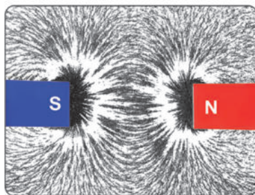
Figure (18) Magnetic field lines between two opposite poles of two magnets
