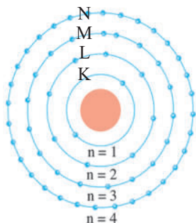
Figure (4) The number of electrons required to saturate the first four energy levels
