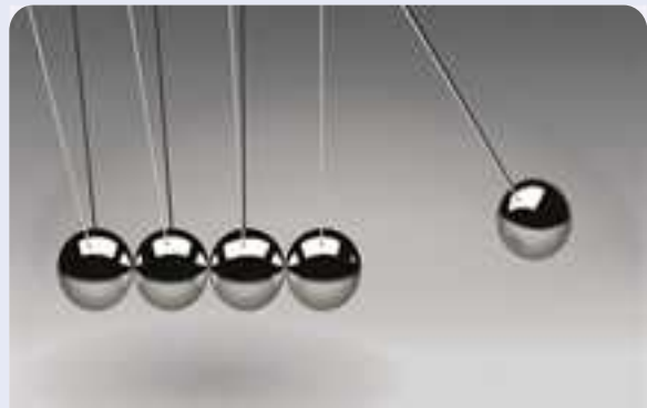
pendulum balls
